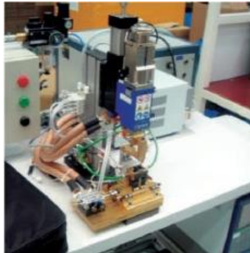
电阻焊治具 Resistance welding fixture
